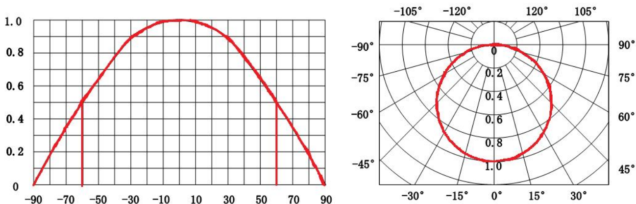
配光曲线 Light distribution curve
