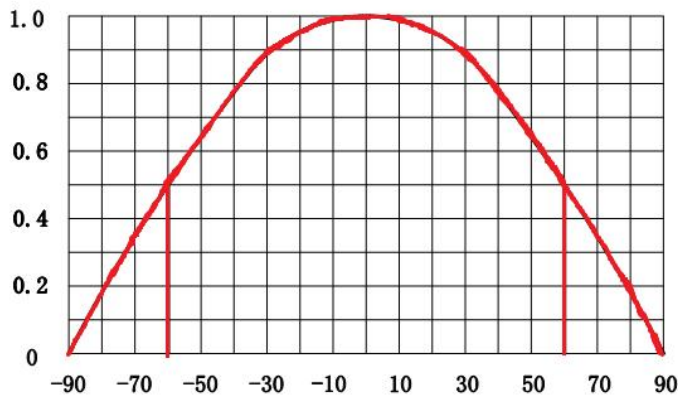
配光曲线 Light distribution curve
