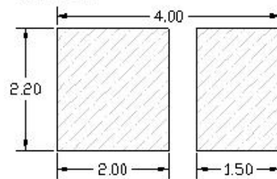
推荐焊盘尺寸 Recommend Pad size
