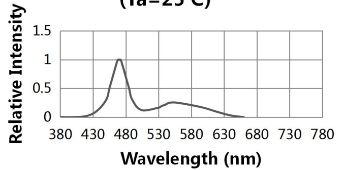
Spectrum Distribution (Ta=25°C)
