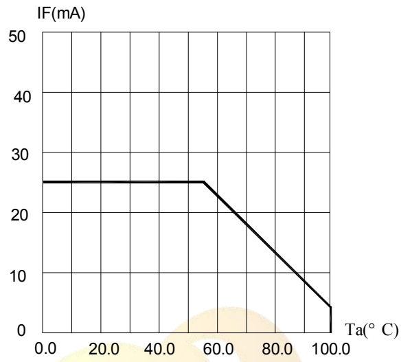
FIG.2 MAXIMUM FORWARD DC CURRENT VS AMBIENT TEMPERATURE(Tjmax=110 ° C)
