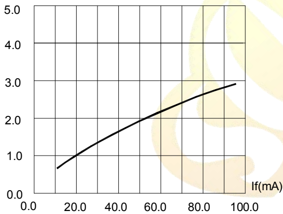
FIG.3 RELATIVE LUMINOUS INTENSITY VS. FORWARD CURRENT
