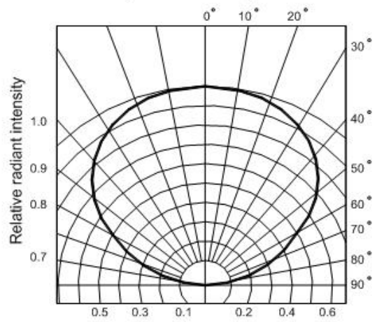
Fig.6 Radiation diagram
