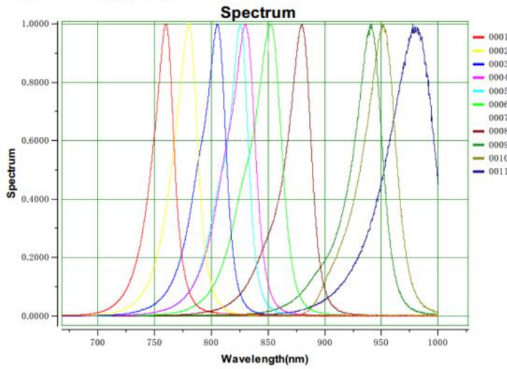
Fig 1. Color Spectrum (光谱图), T_a = 25^\circ\text{C} , RH60%
